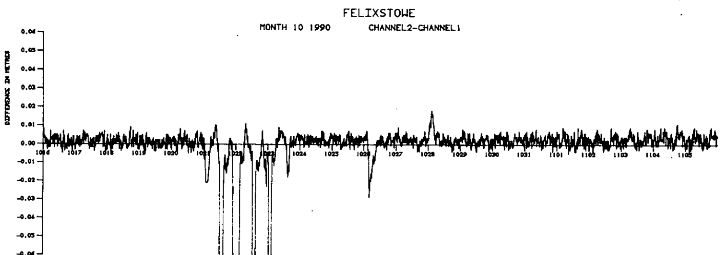
Figure 2. Typical plots of a) Raw Dataring values covering a period of a week, and b) The differences between recording channels at a site with two digiquartz sensors.
